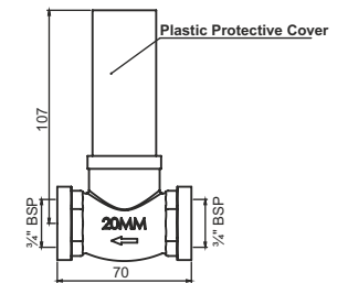
Concealed Stop Valve Body - 20mm
