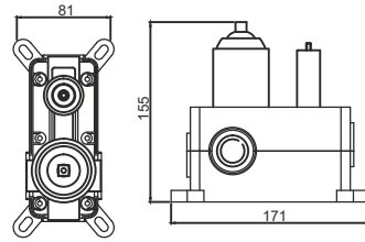
45mm High Flow Single Lever Concealed Diverter Body
